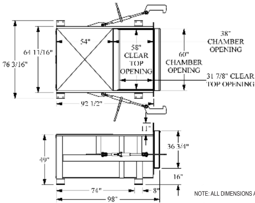
10 HP 44 Gallon Power Unit
