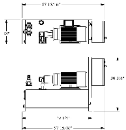
10 HP 44 Gallon Power Unit
